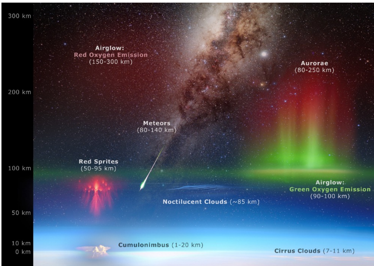
This diagram shows the layers of the Earth's upper atmosphere and the phenomena which occur in them. Credit: P. Horálek /NOIRLab/NSF/AURA
